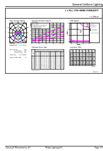
General uniform lighting - 17PL-L/COR/22-840/MF22/G/4P 10/1
