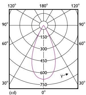
Light Distribution Diagram - RS350 G2 RC Rd D55 4W 30K 50D 1H
