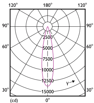
Light Distribution Diagram - RS350 G2 RC Rd D100 23W 40K 24D 1H
