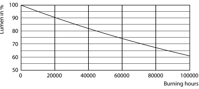
Lumen Maintenance Diagram - MAS LED SON-T IF 9Klm 50W 740 E40
