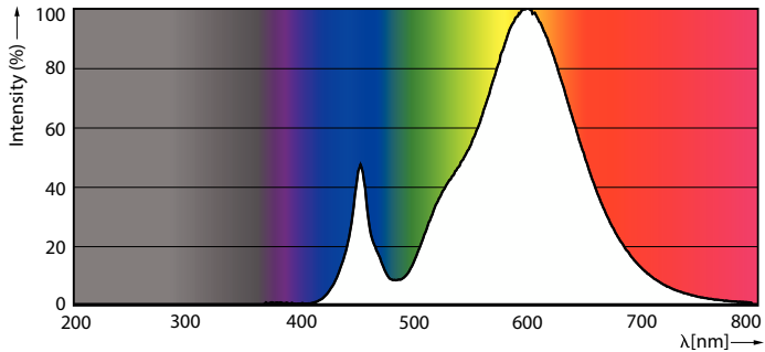
Spectral Power Distribution Colour - MAS LED SON-T EM 10.8Klm 65W 727 E40
