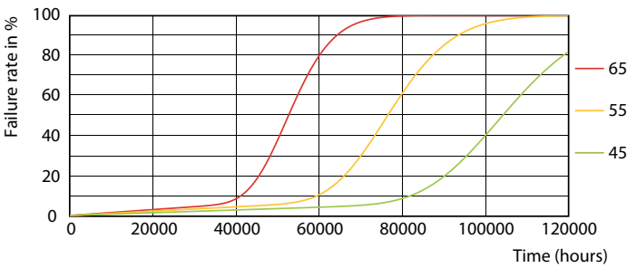
LEDtube-100K-4565-FailureRate-LED
