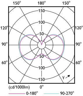
Light Distribution Diagram - 115CC/MAS/850/LS EX39 G2 BB 277-480V 3/1
