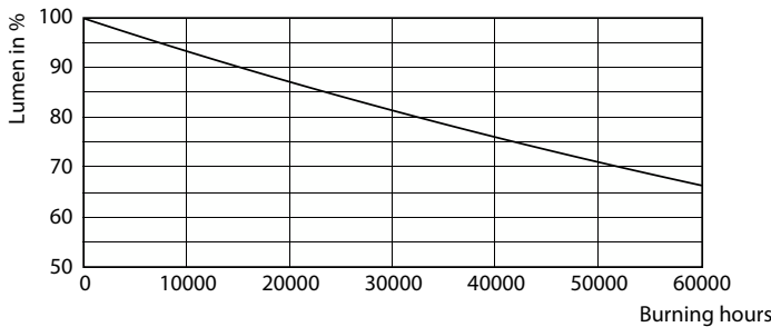
Lumen Maintenance Diagram - 115CC/MAS/850/LS EX39 G2 BB 277-480V 3/1
