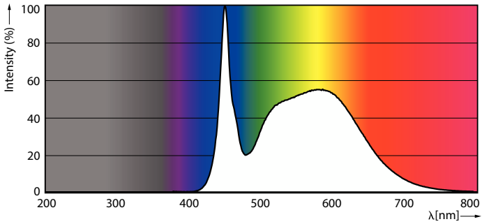
Spectral Power Distribution Colour - 115CC/MAS/850/LS EX39 G2 BB 277-480V 3/1
