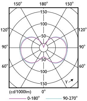
Light Distribution Diagram - 150CC/MAS/840/LS EX39 G2 BB 277-480V 3/1
