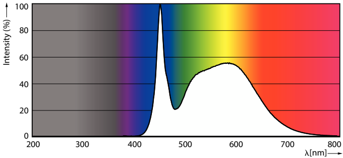
Spectral Power Distribution Colour - 150CC/MAS/850/LS EX39 G2 BB 277-480V 3/1
