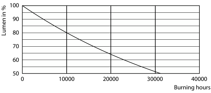
Lumen Maintenance Diagram - MAS VLE LEDBulbD11.2-100W E27 940A60CLG
