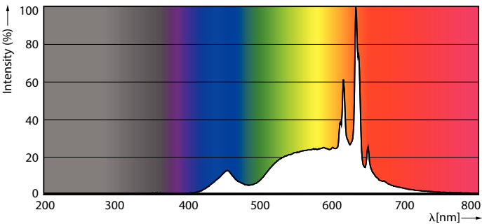
Spectral Power Distribution Colour - CorePro LEDbulb ND 8-60W A60 E27 927 UK
