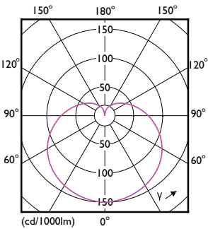
Light Distribution Diagram - CorePro LEDbulb ND 7.5-60W A60 E27 930UK
