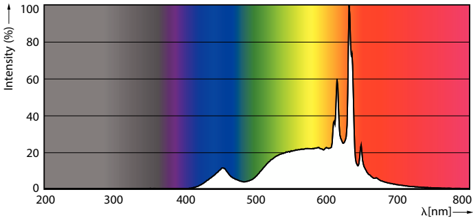
Spectral Power Distribution Colour - CorePro LEDbulb ND 11-75W A60 E27 927 UK
