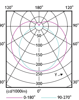
Light Distribution Diagram - MAS LEDtube HF 1200mm UO 16W865 T8
