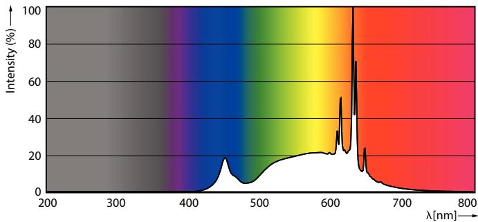
Spectral Power Distribution Colour - 4.5BR30/UE/930/P/E26/D/T20 1PF/3 SRP
