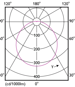
Light Distribution Diagram - 4.5BR30/UE/930/P/E26/D/T20 1PF/3 SRP
