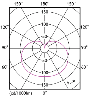
Light Distribution Diagram - 8A19/COR/DipS/5CCT/FR/P/E26/DIM/T20 1CT
