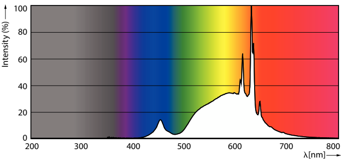
Spectral Power Distribution Colour - LED CLA 4W A60 E27 2700K FR UE SRT6
