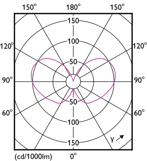
Light Distribution Diagram - LED CLA 4W A60 E27 2700K FR UE SRT6
