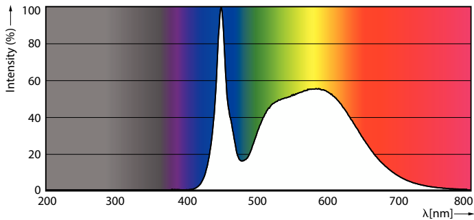
Spectral Power Distribution Colour - 80CC/MAS/3CCT/LS EX39 BB 3/1
