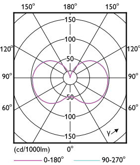
Light Distribution Diagram - 80CC/MAS/3CCT/LS EX39 BB 3/1
