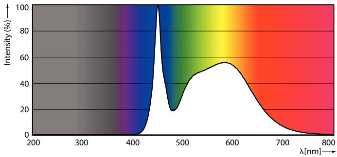
Spectral Power Distribution Colour - 115CC/MAS/3CCT/LS EX39 BB 3/1
