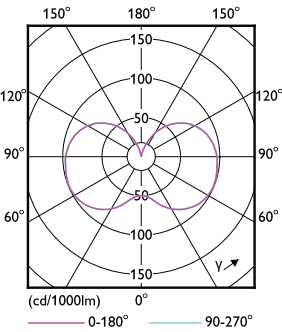
Light Distribution Diagram - 115CC/MAS/3CCT/LS EX39 BB 3/1
