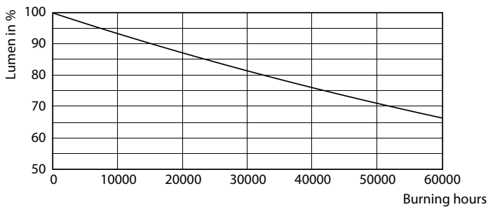
Lumen Maintenance Diagram - 115CC/MAS/3CCT/LS EX39 BB 3/1
