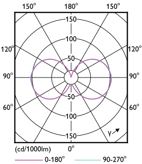
Light Distribution Diagram - 145CC/MAS/3CCT/LS EX39 BB 3/1
