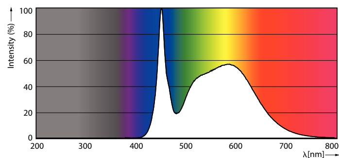
Spectral Power Distribution Colour - 145CC/MAS/3CCT/LS EX39 BB 3/1
