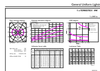
Light Distribution Diagram - MAS LEDBulbND4-60W E27 830 A60 FR G UE
