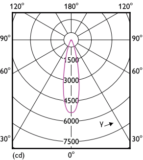
Light Distribution Diagram - 13PAR38/COR/930/F25/DIM/P/ULW/T20 6/1FB
