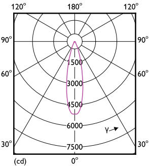
Light Distribution Diagram - 13PAR38/COR/950/F25/DIM/P/ULW/T20 6/1FB
