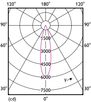
Light Distribution Diagram - 13PAR38/COR/935/F25/DIM/P/ULW/T20 6/1FB
