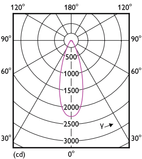
Light Distribution Diagram - 10PAR38/COR/930/F40/DIM/P/ULW/T20 6/1FB
