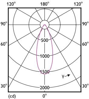
Light Distribution Diagram - 8.5PAR30L/COR/927/F40/D/P/ULW/T20 6/1FB
