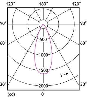
Light Distribution Diagram - 8.5PAR30S/COR/927/F40/D/P/ULW/T20 6/1FB
