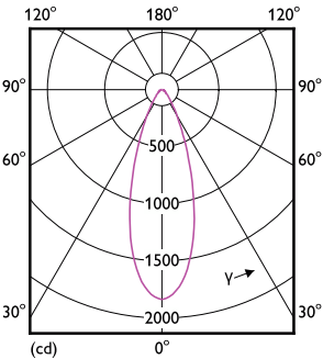
Light Distribution Diagram - 8.5PAR30S/COR/930/F40/D/P/ULW/T20 6/1FB
