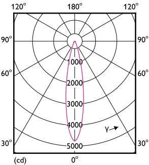
Light Distribution Diagram - 8.5PAR30S/COR/935/F25/D/P/ULW/T20 6/1FB
