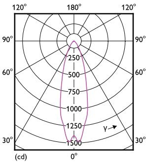
Light Distribution Diagram - 5.5PAR20/COR/F25/930/DIM/P/T20 6/1FB
