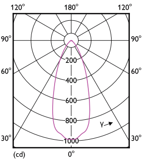
Light Distribution Diagram - 5.5PAR20/COR/F40/930/DIM/P/T20 6/1FB
