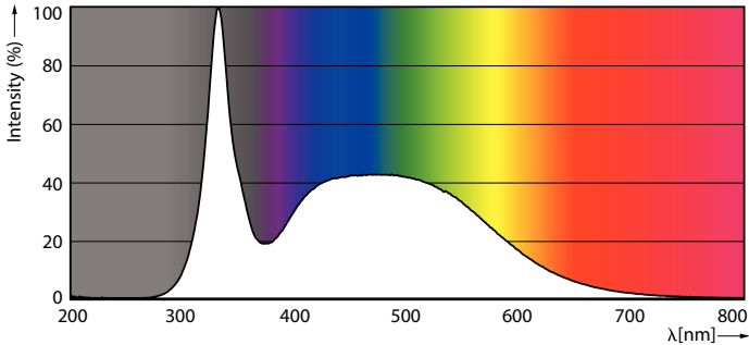
Spectral Power Distribution Colour - CorePro LEDtube 1500mm UO 25.9W 865 T8
