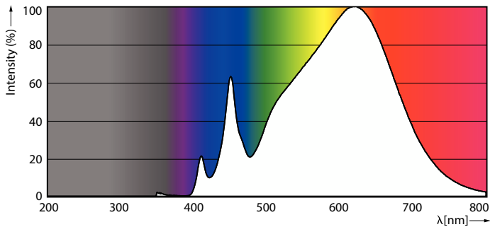
Spectral Power Distribution Colour - 14PAR38/EXPERTCOLOR RETAIL/S8/930/P/D
