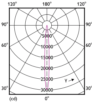
Light Distribution Diagram - 14PAR38/EXPERTCOLOR RETAIL/S8/930/P/D
