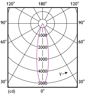
Light Distribution Diagram - 10PAR30L/EXPERTCOLOR RETAIL/S10/930/D
