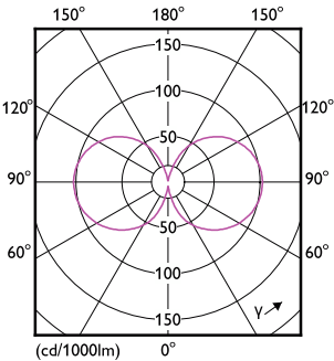
Light Distribution Diagram - 25GC/COR/830/ND E26 BB 6/1
