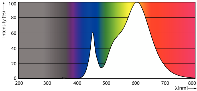
Spectral Power Distribution Colour - 25GC/COR/830/ND E26 BB 6/1
