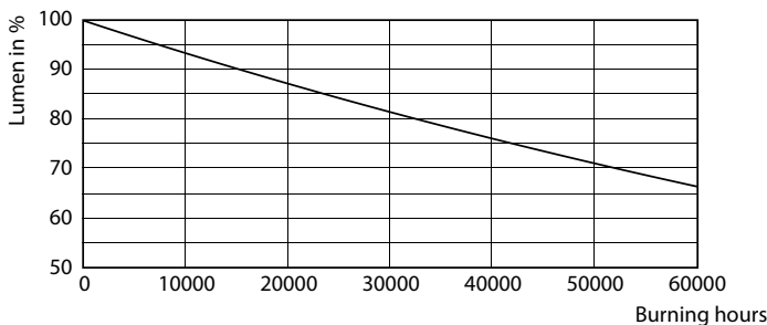
Lumen Maintenance Diagram - 34GC/MAS/830 EX39 BB 6/1
