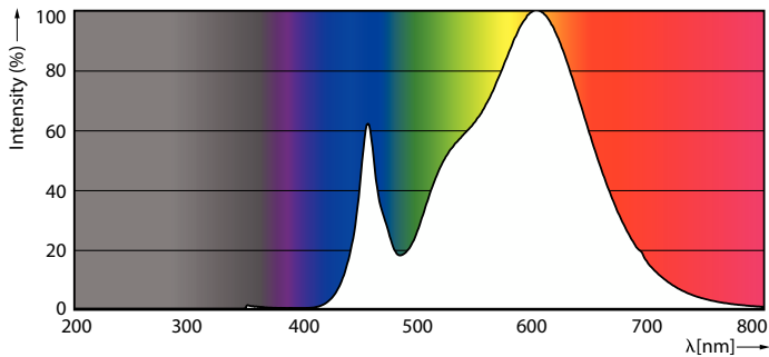
Spectral Power Distribution Colour - 34GC/MAS/830 EX39 BB 6/1
