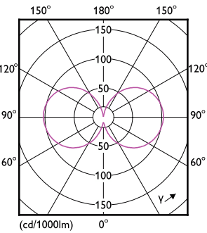
Light Distribution Diagram - 34GC/MAS/830 EX39 BB 6/1
