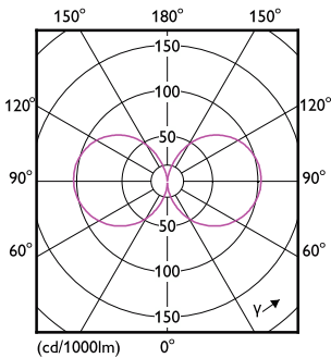
Light Distribution Diagram - 45GC/MAS/850 EX39 BB 6/1
