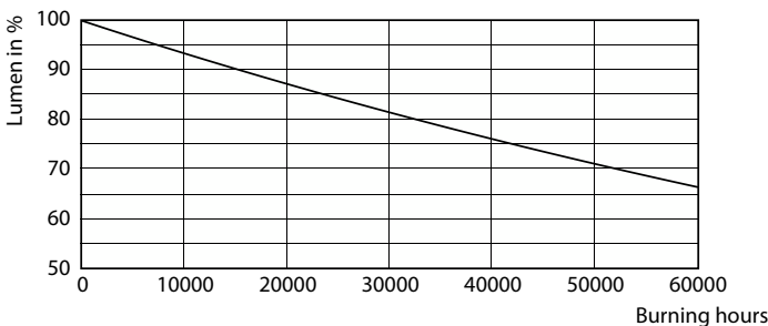
Lumen Maintenance Diagram - 45GC/MAS/850 EX39 BB 6/1
