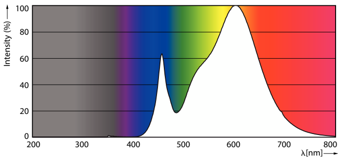
Spectral Power Distribution Colour - 54GC/MAS/830 EX39 BB 6/1
