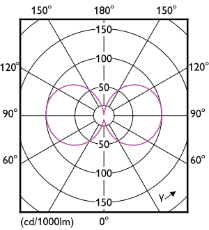
Light Distribution Diagram - 54GC/MAS/830 EX39 BB 6/1
