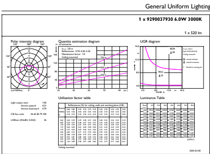
Light Distribution Diagram - EcoHome LEDBulb 6W E27 3000KHV 1PF/20AR
