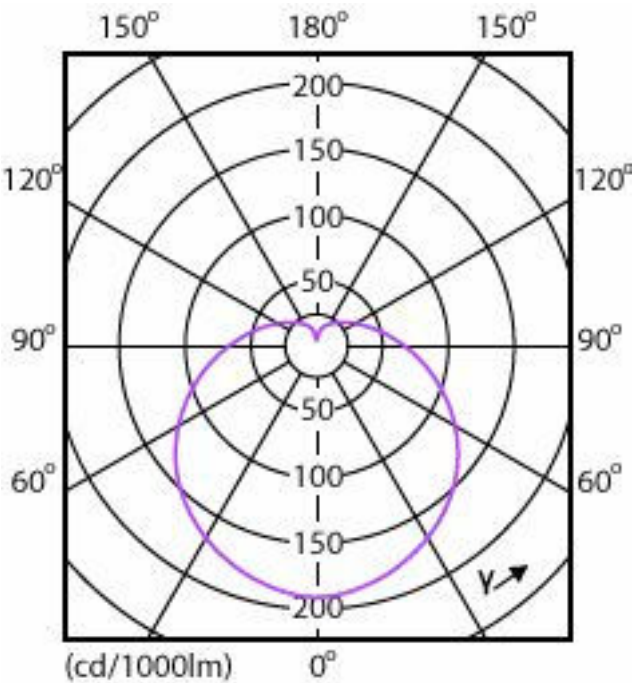
Light Distribution Diagram - EcoHome LEDBulb 6W E27 6500KHV 1PF/20AR
