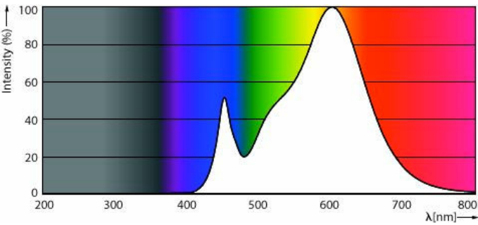
Spectral Power Distribution Colour - EcoHome LEDBulb 8W E27 3000KHV 1PF/20AR
