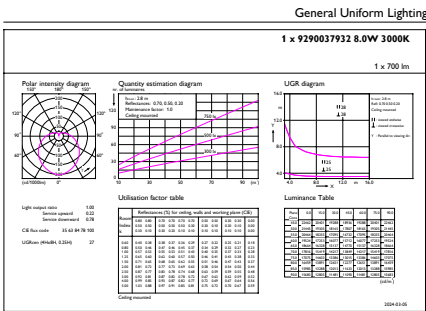
Light Distribution Diagram - EcoHome LEDBulb 8W E27 3000KHV 1PF/20AR
