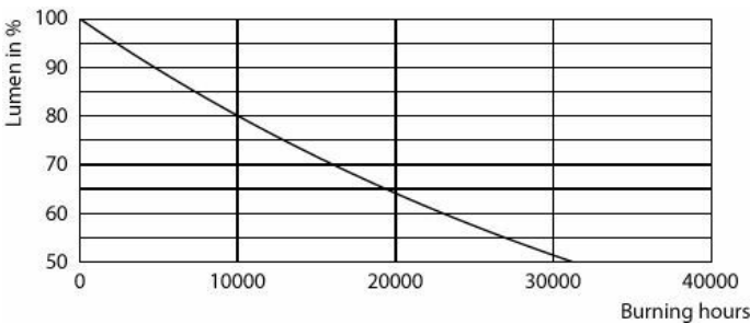
Lumen Maintenance Diagram - EcoHome LEDBulb 8W E27 3000KHV 1PF/20AR
