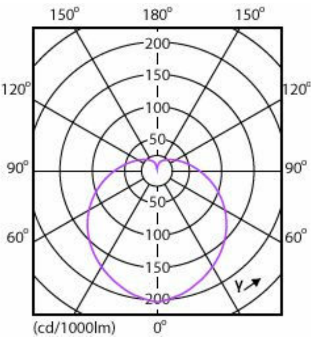
Light Distribution Diagram - EcoHome LEDBulb 8W E27 3000KHV 1PF/20AR
