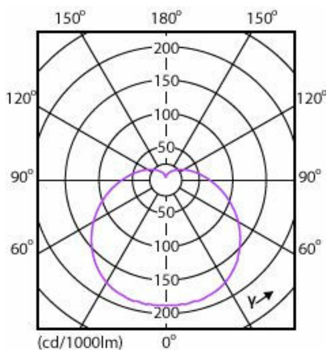
Light Distribution Diagram - EcoHome LEDBulb 10.5WE27 3000KHV1PF/20AR
