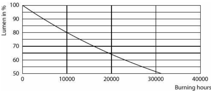
Lumen Maintenance Diagram - EcoHome LEDBulb 10.5WE27 3000KHV1PF/20AR
