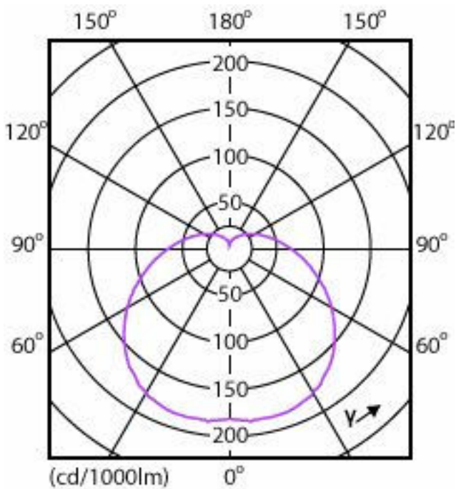
Light Distribution Diagram - EcoHome LEDBulb 13W E27 3000KHV 1PF/20AR
