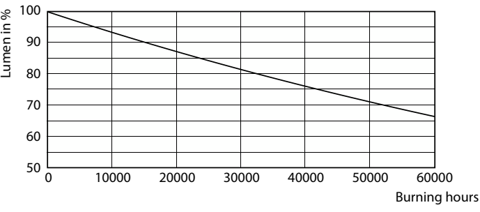
Lumen Maintenance Diagram - MAS LEDspot UE 2.1-50W GU10 DIM 827 EELA
