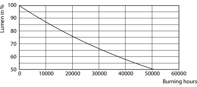
Lumen Maintenance Diagram - MAS LEDBulb DT7.2-75W E27 CRI95A60CL G
