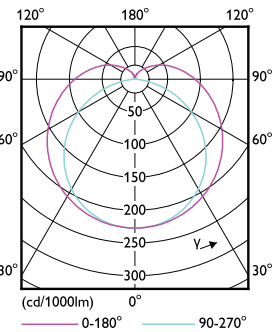
Light Distribution Diagram - MAS LEDtube 1200mm HO 11.3W 865 T8 EELB
