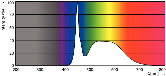
Spectral Power Distribution Colour - MAS LEDtube 1200mm HO 11.3W 865 T8 EELB
