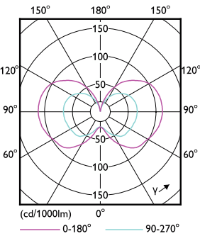
Light Distribution Diagram - 18-12-9CC/COR/3PW/3CCT/E26 BB 6/1
