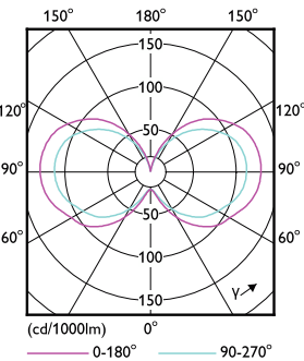
Light Distribution Diagram - 27-18-12CC/COR/3PW/3CCT/E26 BB 6/1
