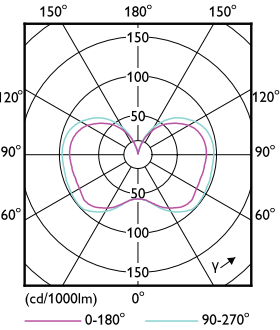
Light Distribution Diagram - 36-27-18CC/COR/3PW/3CCT/E26 BB 6/1
