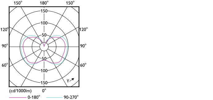
Light Distribution Diagram - 36-27-18CC/MAS/3PW/3CCT/Ex39 BB 3/1
